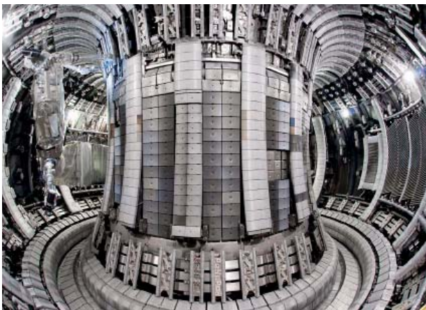
Figure 1.9: Inside of JET following the shutdown.
