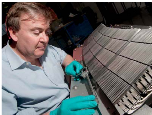
Figure 1.8: Final fit check of bulk tungsten tiles on a jig, carried out by Philippe Mertens from FZ Jülich.
