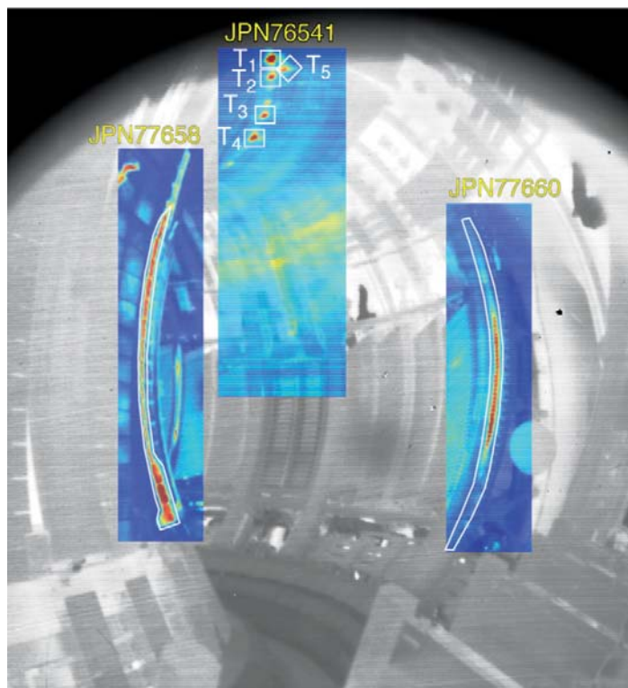
Figure 1.12: Plasma facing components in JET as seen by the wide angle view infrared camera. The coloured areas are examples illustrating the regions of interest selected for fast time resolution measurement (1 millisecond): the upper dump plate where runaway electrons cause local hot spots (JET Pulse Number 76541), the inner limiter (JET Pulse Number 77658) and the outer limiter (JET Pulse Number 77660).
