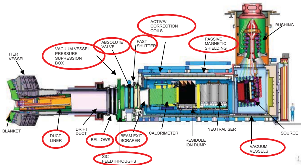
Figure 1.24: With CIEMAT (Spain) as third party, CCFE has an F4E grant to design the components which will integrate the neutral beam system with the ITER assembly. In this picture of the beam-line, the integration subsystems are highlighted. In other neutral beam work, CCFE is third party to the Italian RFX consortium for the design of components for the MITICA neutral beam test bed to be built in Italy.
