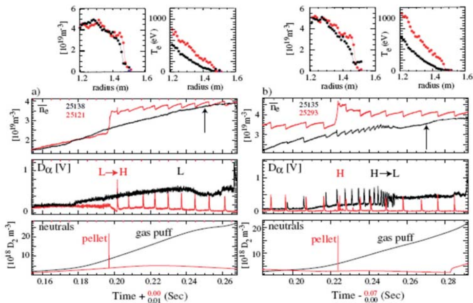
Figure 1.14: Effect of fuelling method on L-H (a) and H-L (b) transition. High field side pellet (red) and low field side gas puff (black) were used. Top panels show edge electron density and temperature profiles at times indicated by arrows. Note time offsets.
