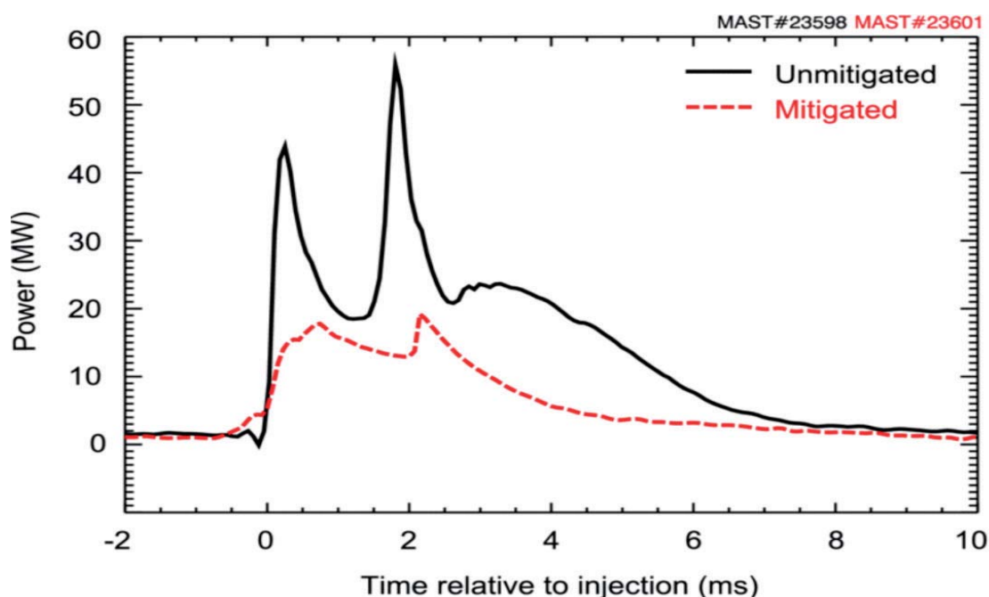
Figure 1.15: Total power load delivered to the divertor during disruptions on MAST. The dashed red line shows the power load in a mitigated disruption and the solid black line shows the power load in an unmitigated disruption.
