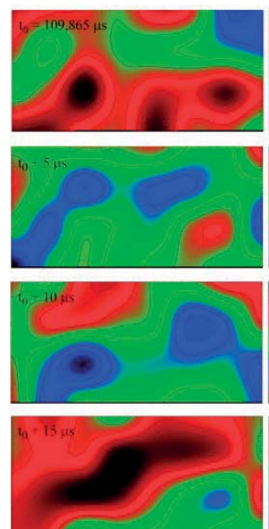
Images of plasma turbulence produced by MAST's new Beam Emission Spectroscopy diagnostic.
