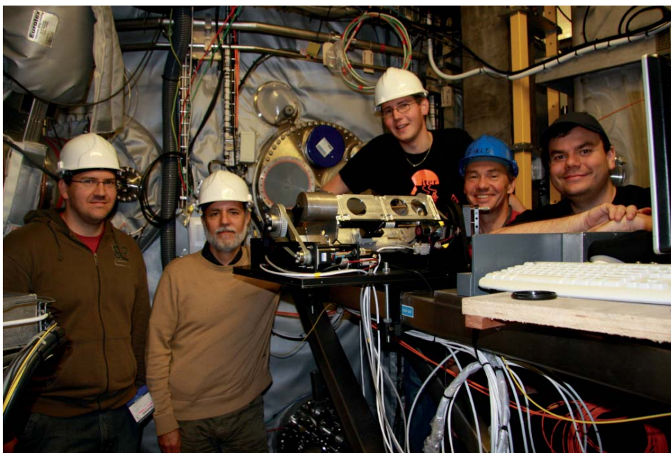
Figure 1.13: Members of the Hungarian and CCFE team responsible for the new Beam Emission Spectroscopy diagnostic, with the external optical system during installation on MAST in June 2010.
