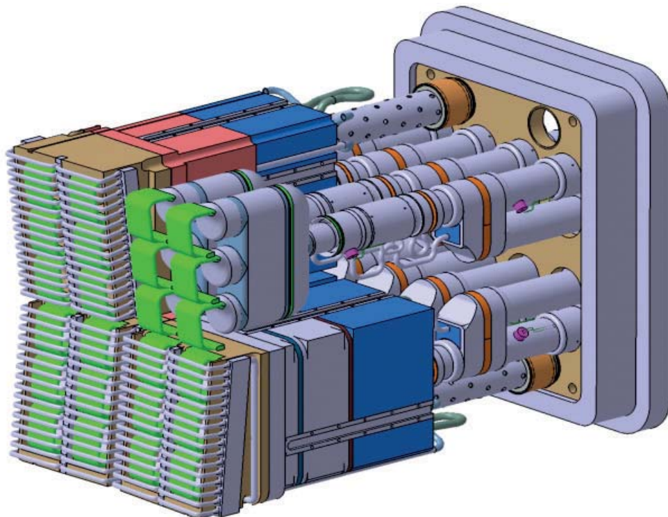
Figure 1.23: Model of the ITER ICRF Antenna design as at March 2011. In 2010/11, development of this 3D CATIA model concentrated on the front housing and the Removable Vacuum Transmission Lines. The antenna straps that will face the ITER plasma are to the left of the picture. CCFE leads the consortium comprising the design team which is located at Culham (the other members are from Belgium and France).
