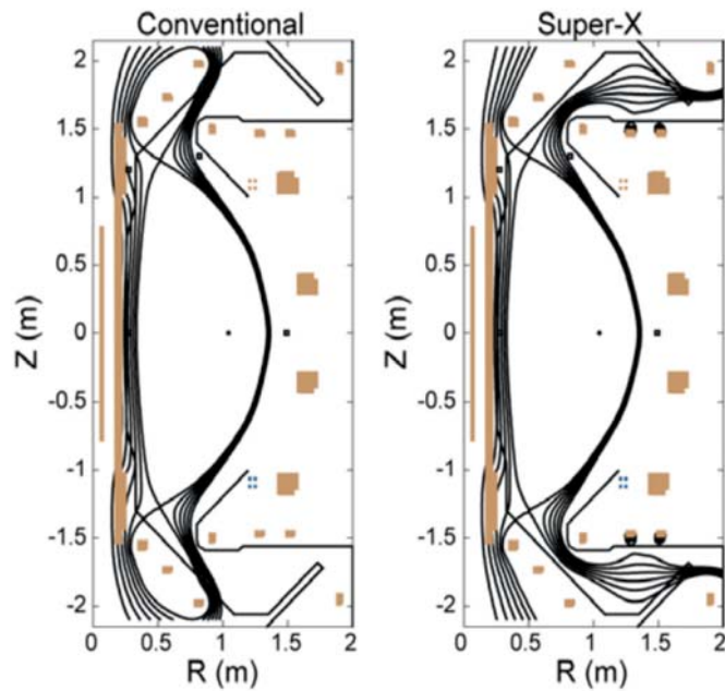
Figure 1.17: Conventional (left hand side) and Super-X (right hand side) configurations achievable with the upgraded MAST Poloidal Field coil set. In the latter, the divertor coils sweep the divertor plume out to large major radius, resulting in decreased power densities at the divertor target tiles.
