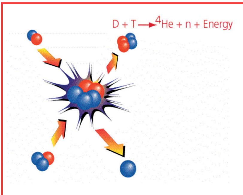
Figure 1.1: The deuterium - tritium fusion reaction produces a helium nucleus (alpha particle) and a neutron. Deuterium and tritium are 'heavy' and 'super-heavy' hydrogen.
