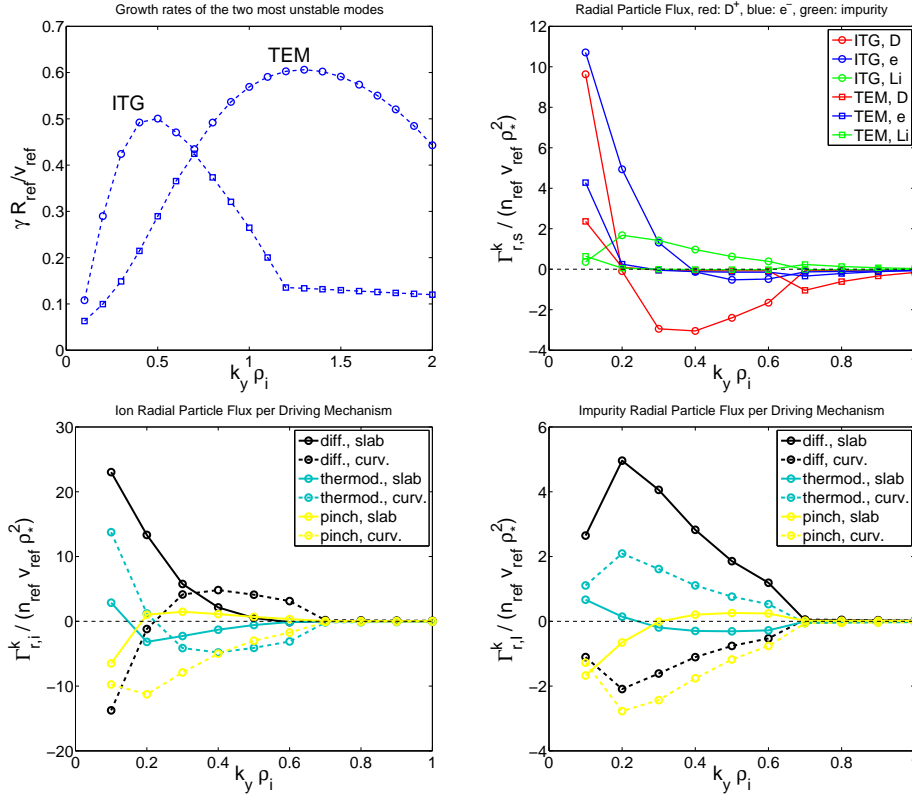
Figure 10. Fluid analysis at t = 0.3\text{s} with the reference c_{\text{Li}} = 0.15 lithium concentration. Growth rates of the two most unstable modes (ITG and TEM, top left), total flux of the species driven by ITG and TE modes (top right), deuterium (bottom left) and lithium (bottom right) particle flux by slab (solid) and curvature (dashed) terms of the diffusive (black), thermo-diffusive (cyan) and pinch (yellow) contributions driven by ITG modes as a function of the bi-normal wavenumber.
