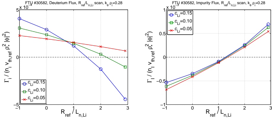
Figure 3. Impurity concentration and impurity density gradient scan of the quasi-linear deuterium (left) and lithium (right) fluxes at t = 0.3s and k_{\theta} \rho_i = 0.28 .
