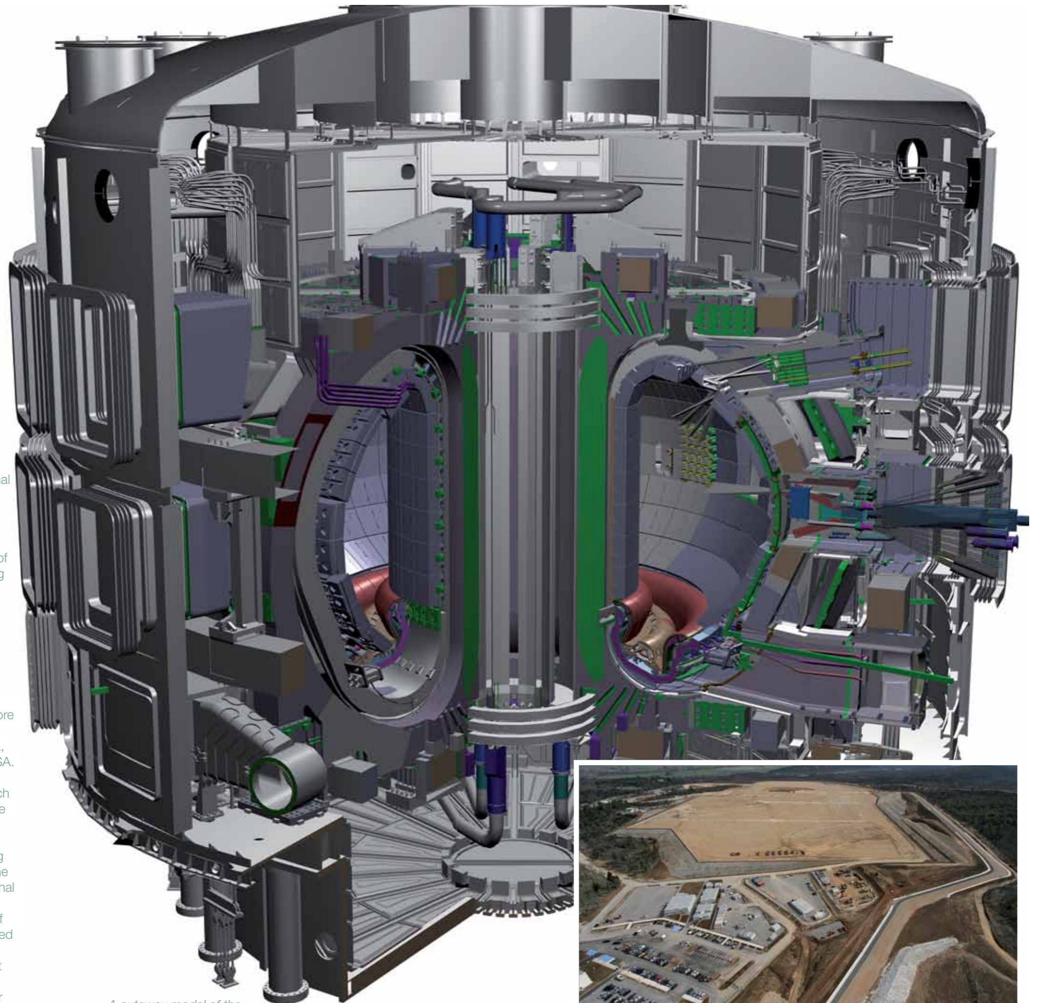
A cutaway model of the ITER tokamak
